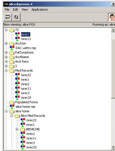
Figure 8: Example hierarchical visualization of a user access rights directed acyclic graph.
