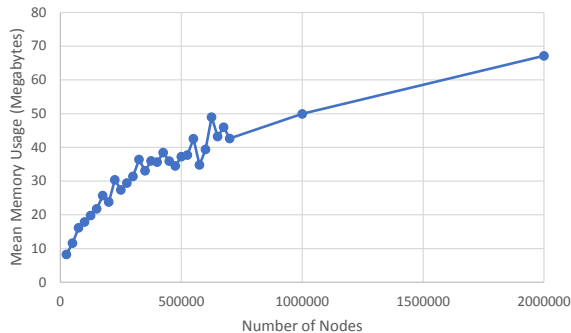
Figure 5: Mean memory usage of the PReview algorithm on graphs up to 2000000 nodes with 50 trials per data point.
