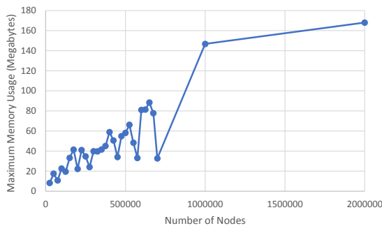
Figure 6: Maximum memory usage of the PREview algorithm on graphs up to 2,000,000 nodes with 50 trials per data point.
