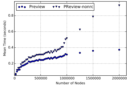
Figure 4: Execution time on graphs up to 2000000 nodes.
