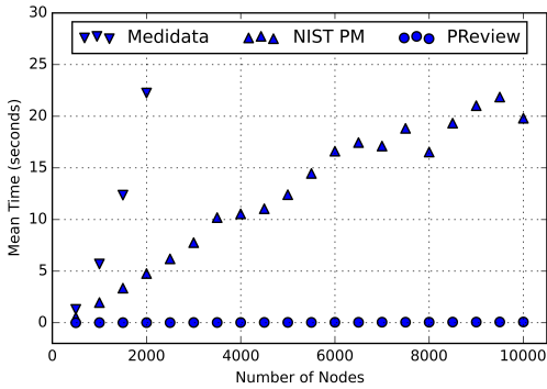
Figure 3: Execution time on graphs up to 10000 nodes.
