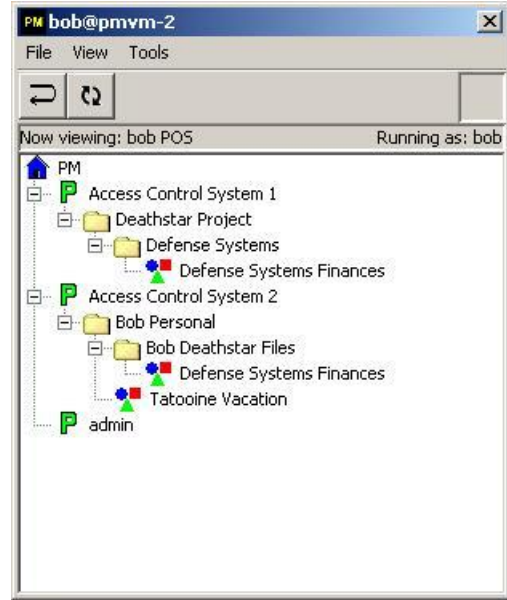
Figure 10: NIST PM File Hierarchy for Access Control Graph in Figure 2.
