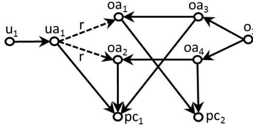
Figure 11: Minimal Access Control Graph Containing an Orphaned File.
