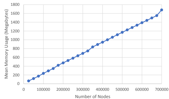
Figure 7: Mean memory consumed by the generated access control graphs up to 700,000 nodes with 50 trials per data point.
