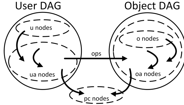
Figure 1: A rough diagram of edge and node relationships for the access control graph.
