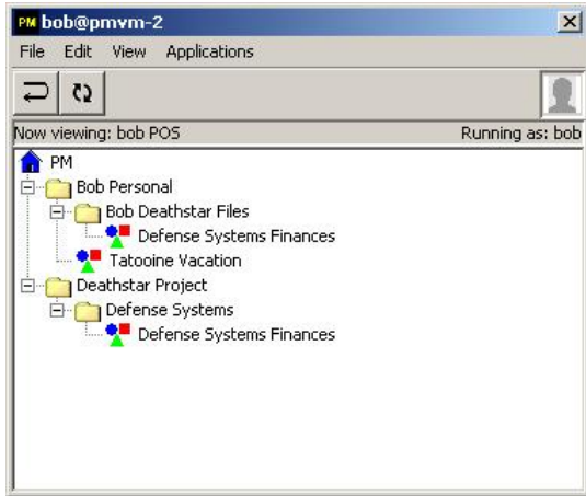
Figure 9: Example File Hierarchy for Access Control Graph in Figure 2.
